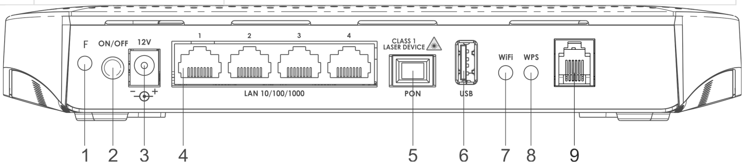
Figure 8 – NTU-RG5421G-Wac rev.B and NTU-RG5421G-WZ rev.B rear panel layout
