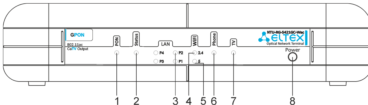
Figure 11 – NTU-RG-5421GC-Wac front panel layout
