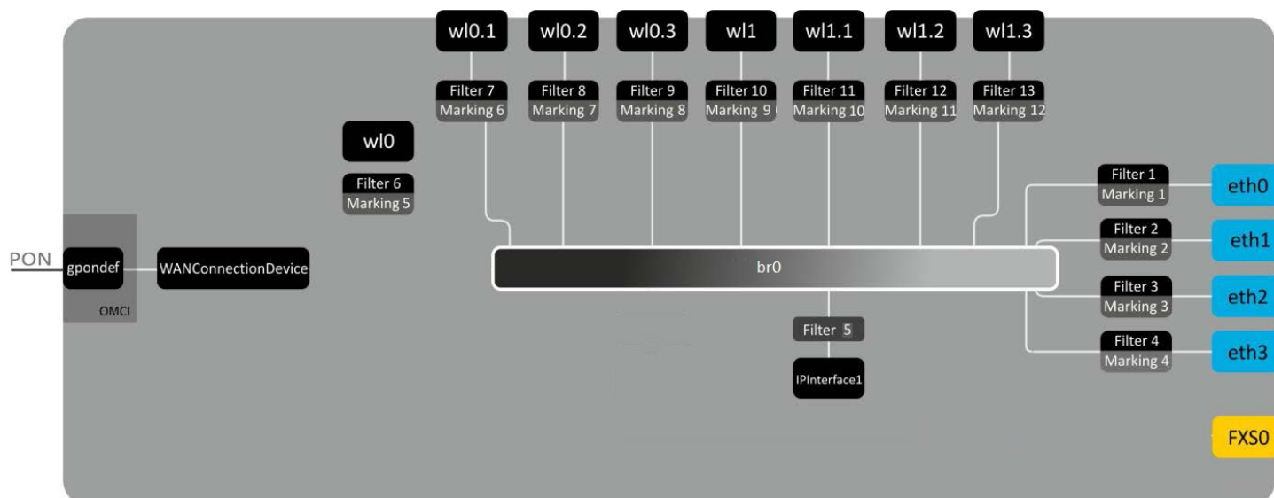
Figure 14 – Logical Architecture of a Device with Factory Settings
