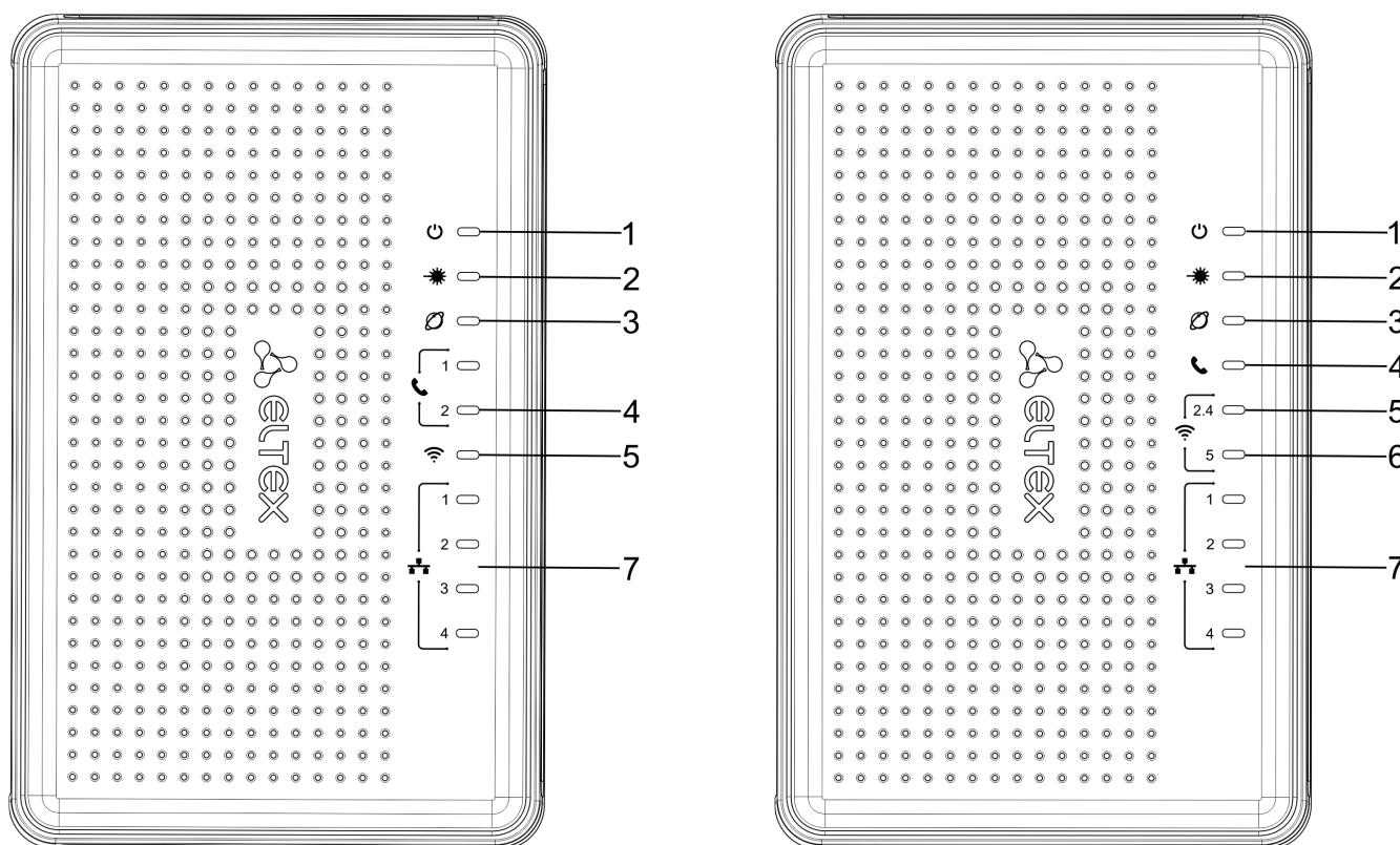
Figure 10 – NTU-RG-5402G-W (on the left) and NTU-RG-5421G-Wac, NTU-RG-5421G-WZ (on the right) top panel layout
