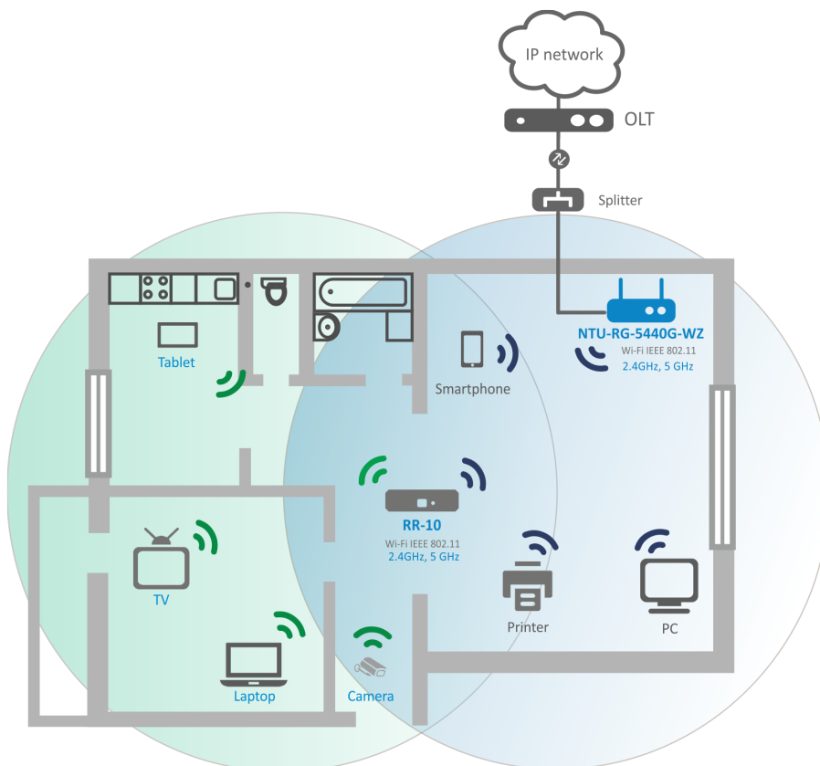
Figure 3 – NTU-RG-5420G-Wac, NTU-RG-5420G-WZ, NTU-RG-5421G-Wac, NTU-RG-5421G-WZ, NTU-RG-5421GC-Wac, NTU-RG-5440G-WZ, NTU-RG-5440G-Wac, NTU-RG-5421G-Wac rev.B, NTU-RG-5421G-WZ rev.B, NTU-RG-5440G-WZ rev.B и NTU-RG-5440G-Wac rev.B application diagram
