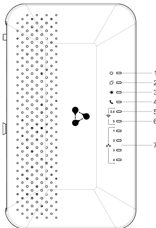
Figure 13 – NTU-RG-5421G-Wac rev.B and NTU-RG-5421G-WZ rev. B top panel layout
