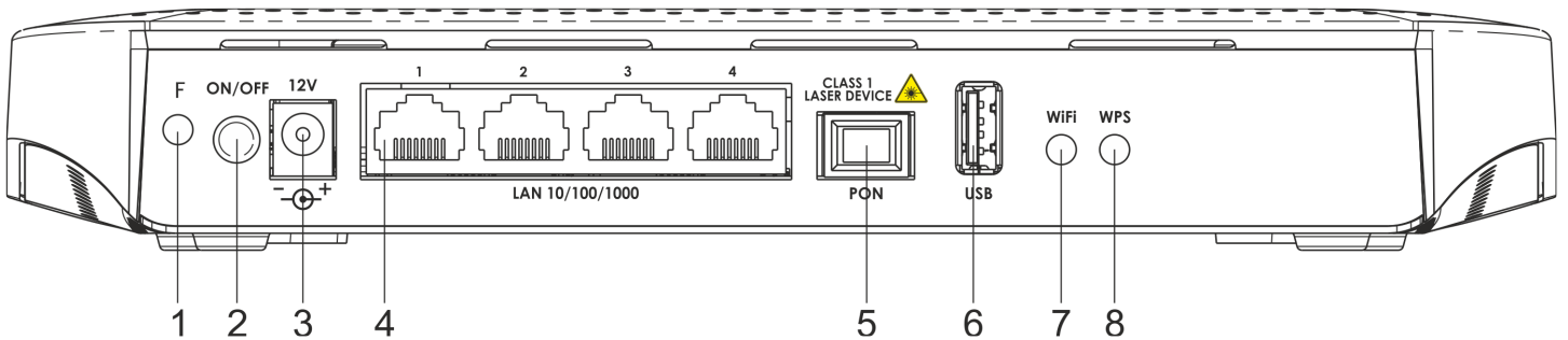
Figure 7 – NTU-RG-5440G-Wac, NTU-RG-5440G-WZ, NTU-RG5420G-Wac, NTU-RG5420G-WZ, NTU-RG5440G-Wac rev.B, NTU-RG5440G-WZ rev.B rear panel layout
