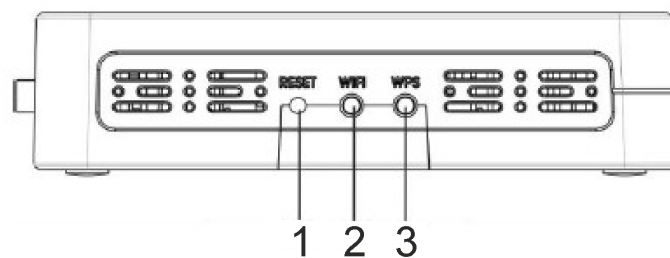
Figure 9 – NTU-RG-5402G-W, NTU-RG-5421G-Wac and NTU-RG-5421G-WZ side panel layout
